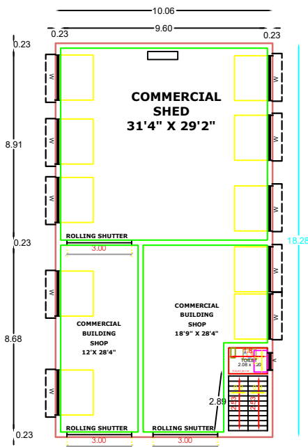
PRO GROUND FLOOR COMMERCIAL BUILDING PLAN
