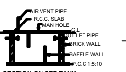
SECTION ON SEPT TANK
