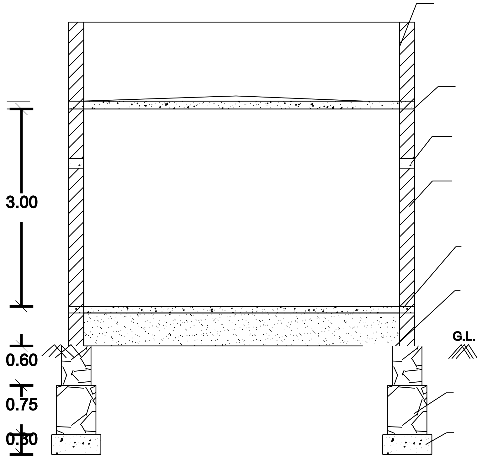
CROSS SECTION
