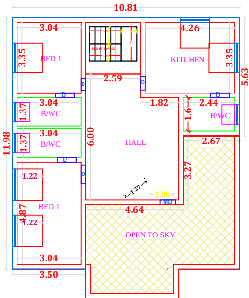
PLAN - FIRST FLOOR PROPOSED
