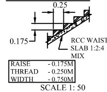
STAIR CASE DETAILS
