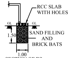
SECTION OF BS
