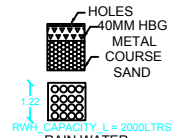
RAIN WATER COLLECTING TANK
