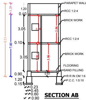
SECTION AB
