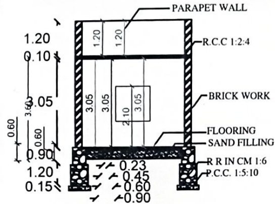
SECTION AB
