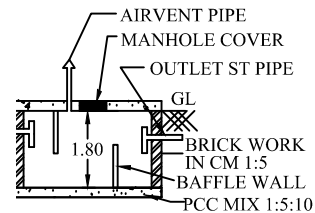
SECTION ON SEPTICTANK
