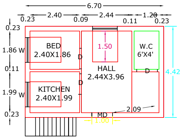
GROUND FLOOR RESIDENTIAL PLAN
