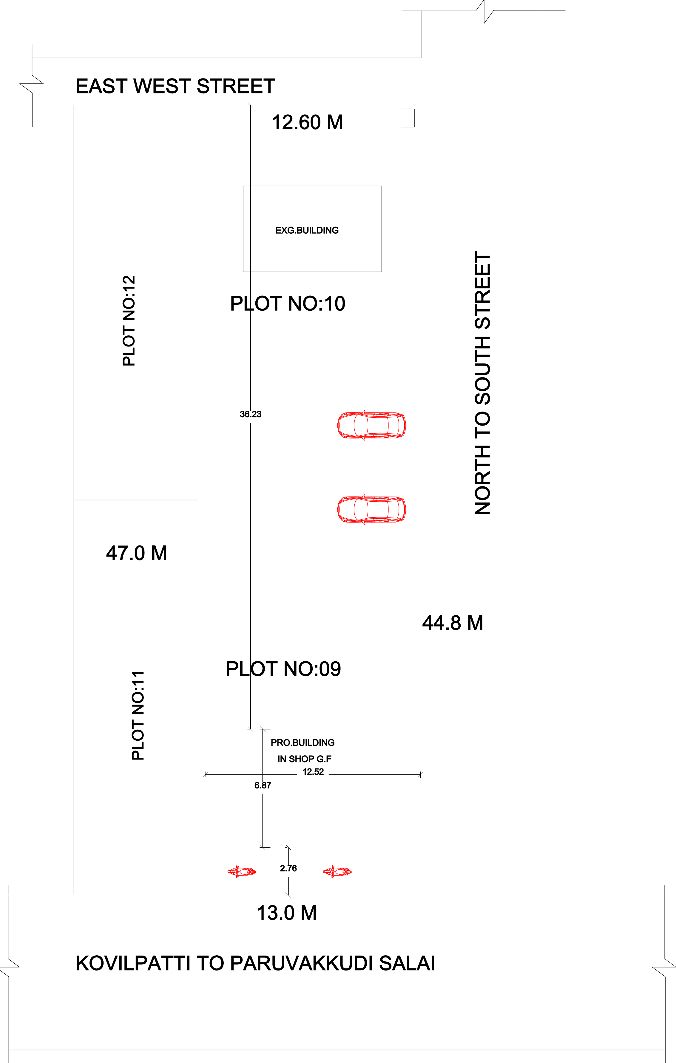
SITE PLAN
