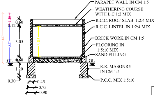
SECTION OF "AB"
