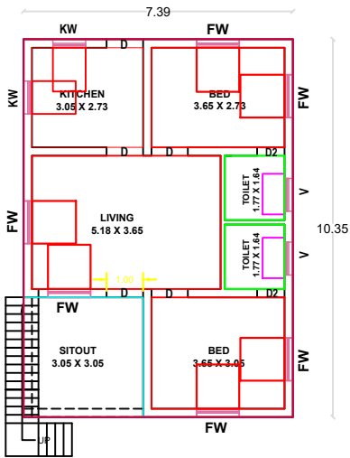
PLAN - GROUND FLOOR ( PROPOSED )
