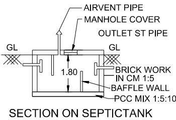
SECTION ON SEPTICTANK
