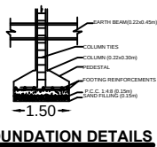
FOUNDATION DETAILS
