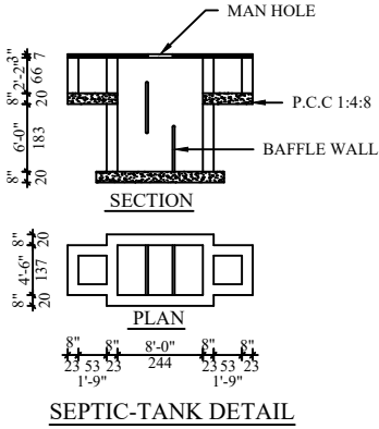
SEPTIC-TANK DETAIL
