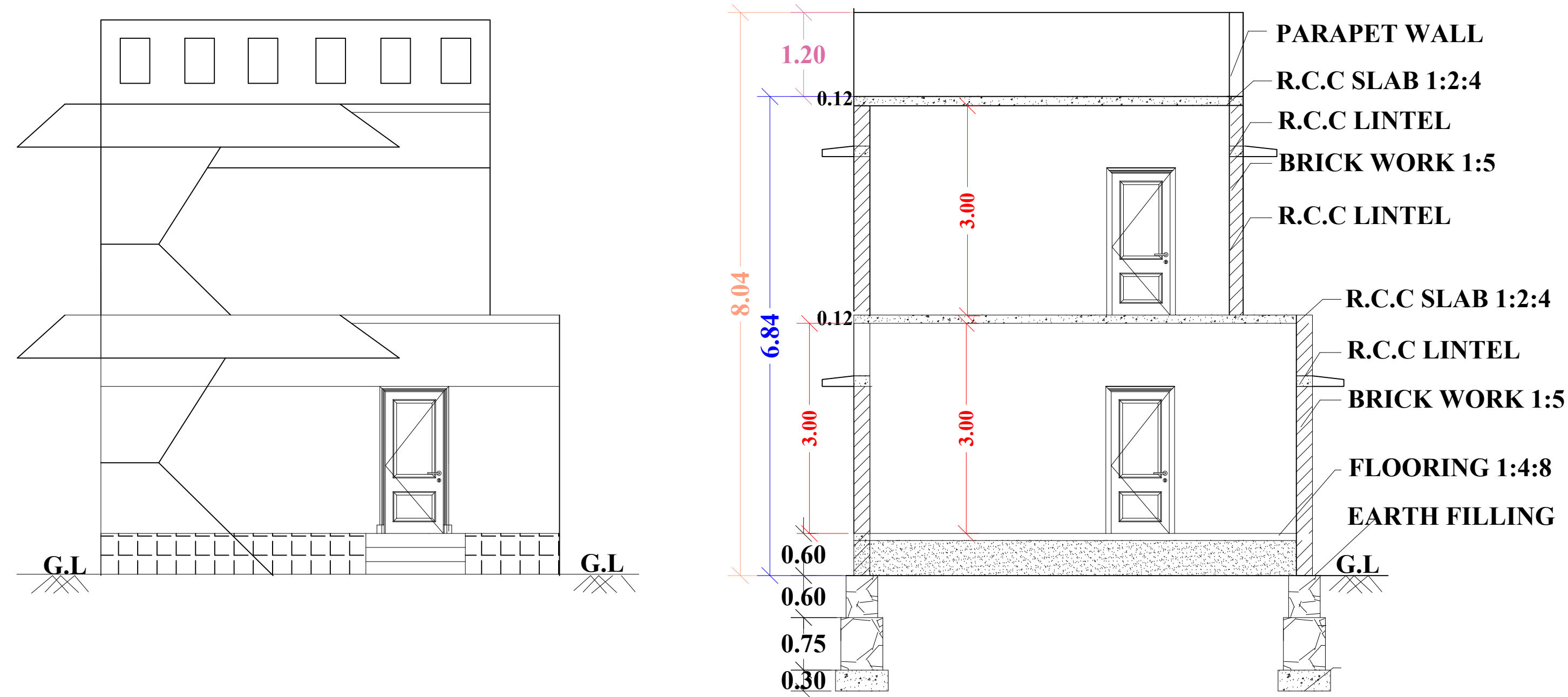
"SECTION "AB"
