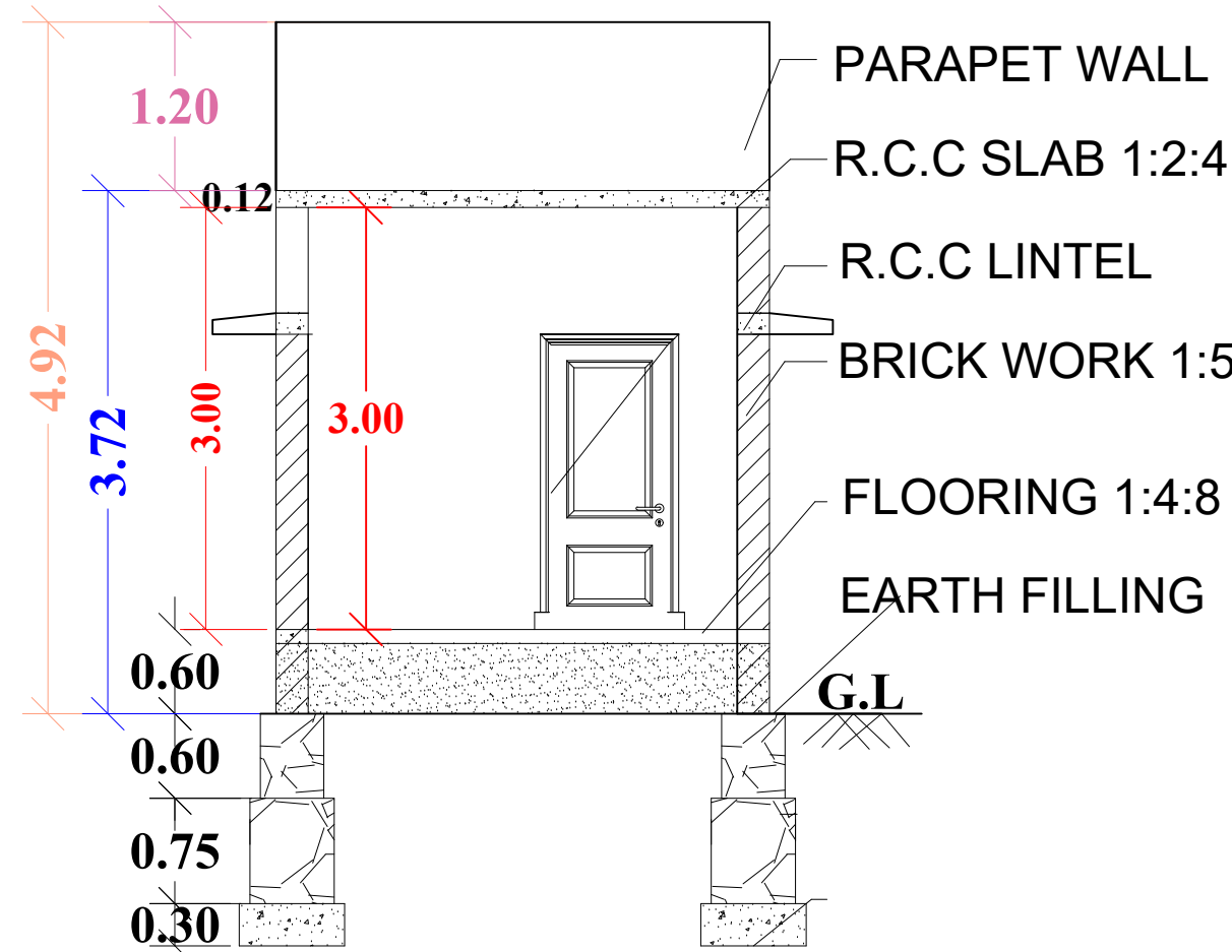
"SECTION "AB"
