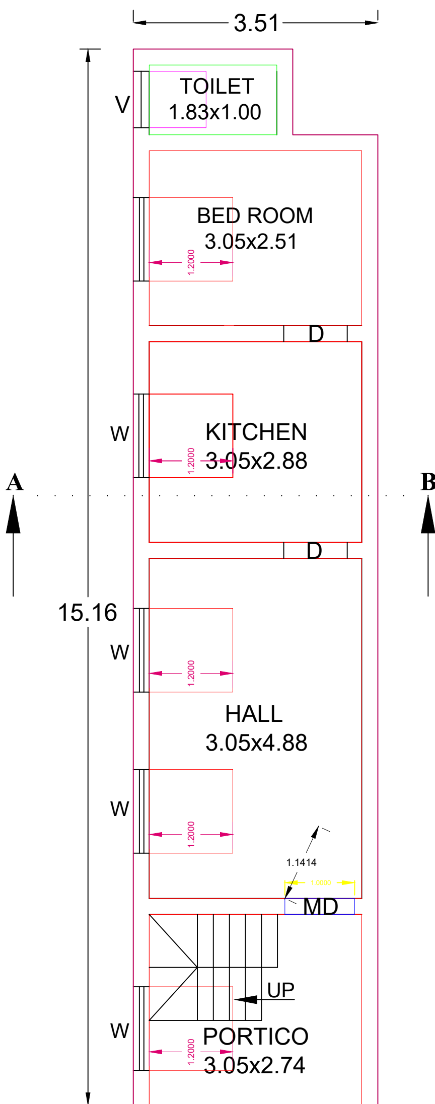
PLAN
