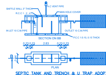
SEPTIC TANK AND TRENCH & U TRAP ADOPTED
