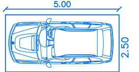
CAR POCKET DETAILS
