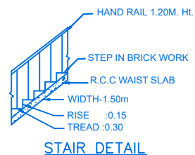
STAIR DETAIL
