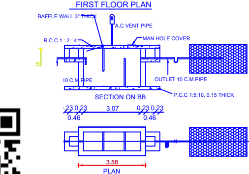
TIC TANK AND TRENCH & U TRAP ADOPTED
