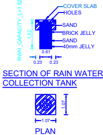
SECTION OF RAIN WATER COLLECTION TANK
