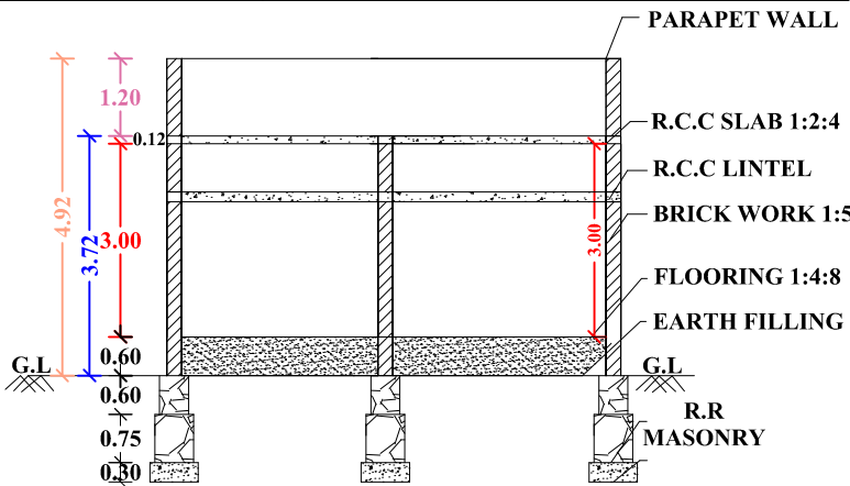
"SECTION "AB"
