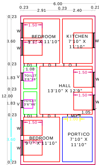
GROUND FLOOR RESIDENTIAL PLAN
