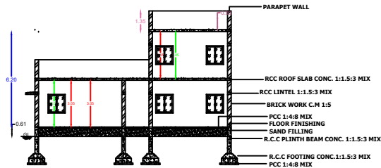
SECTION AB
