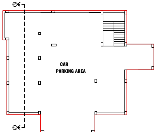
STILT FLOOR
