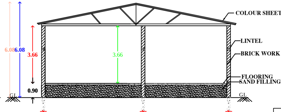
"SECTION "AB"
