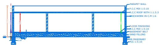
SECTION ON 'XX'
