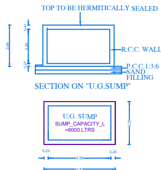
SECTION OF RAIN WATER COLLECTION TANK
