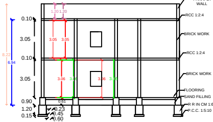
SECTION AB
