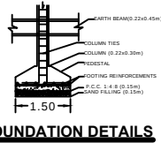
FOUNDATION DETAILS
