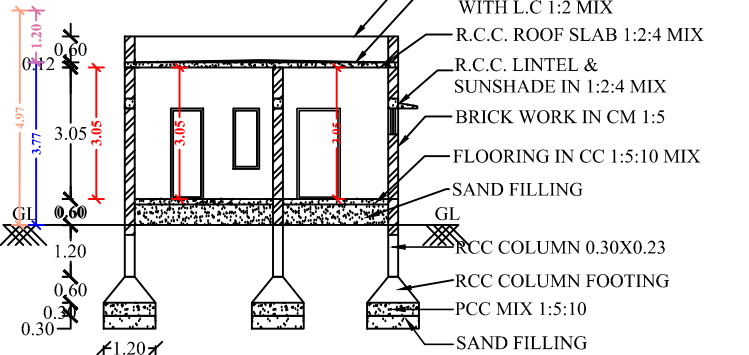
SECTION OF "AB"
