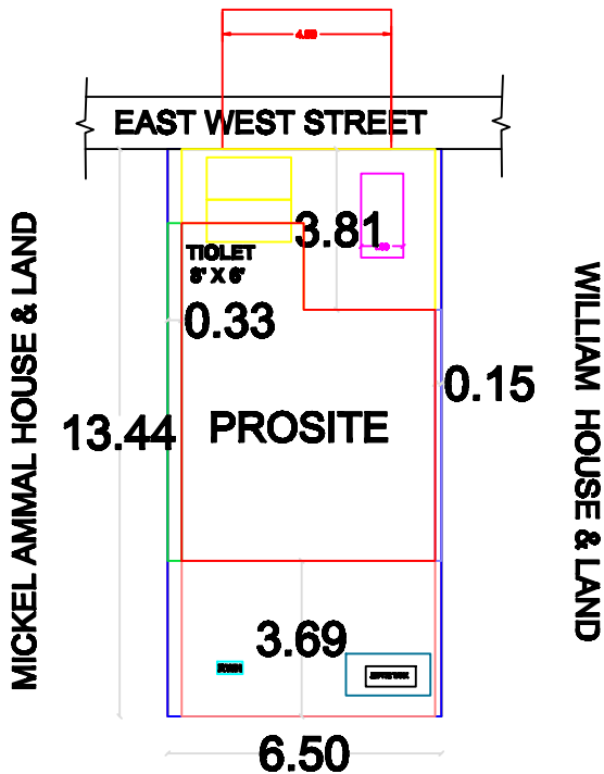
TOPO PLAN
