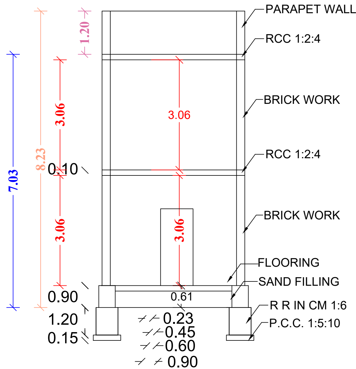
SECTION AB
