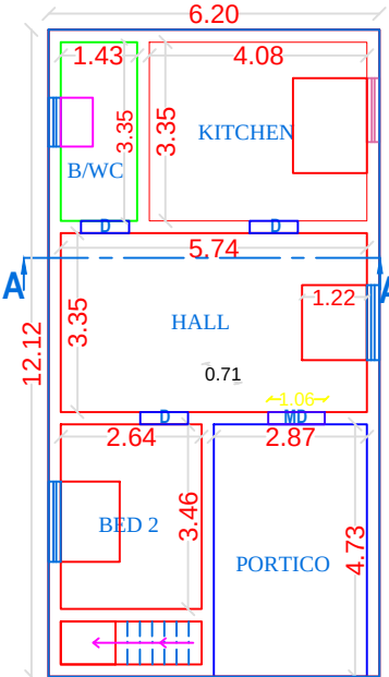
PLAN - GROUND FLOOR ( PROPOSED )
