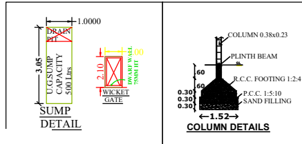
JOURNERY DETAILS
