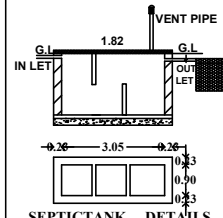
SEPTICTANK DETAILS
