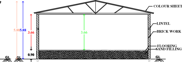
"SECTION "AB"
