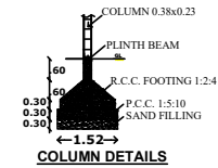
COLUMN DETAILS
