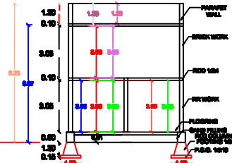
SECTION AB
