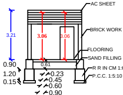
SECTION AB
