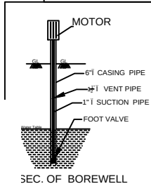
SEC. OF BOREWELL
