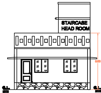
ELEVATION 6.79
