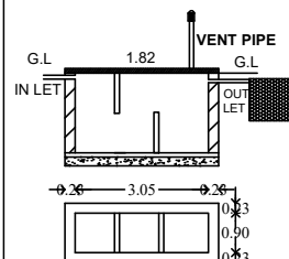
SEPTICTANK DETAILS
