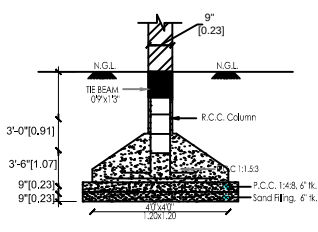
FOUNDATION DETAIL
