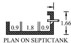
PLAN ON SEPTICTANK
