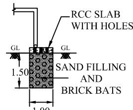
SECTION OF BS
