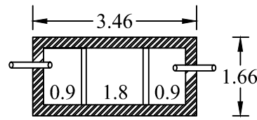
PLAN ON SEPTICTANK
