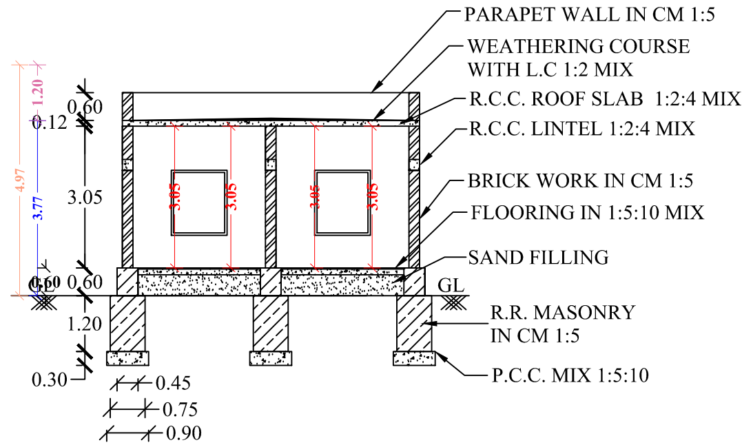
SECTION OF "AB"
