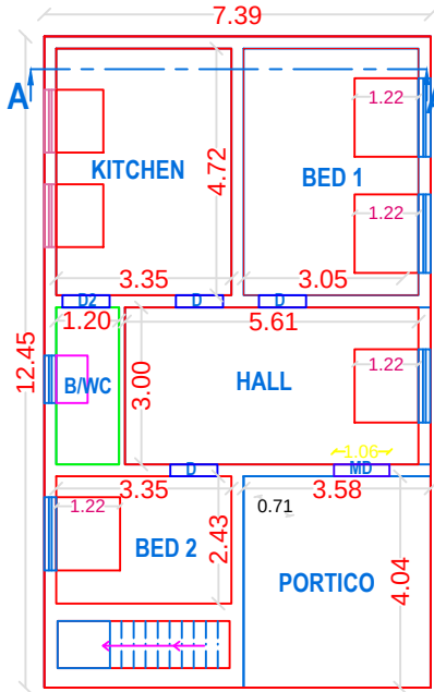
PLAN - GROUND FLOOR (PROPOSED)
