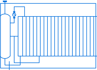
SOLAR PANEL FOR HEATING SYSTEM
