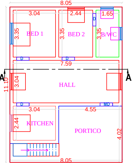
PLAN - GROUND FLOOR PROPOSED
