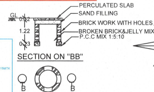
PLAN OF PERCULATION PIT FOR 30 SQ.M
