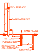
RAIN WATER HARVESTING SYSTEM
