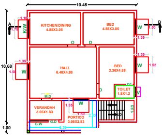
GROUND FL
