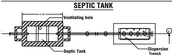
PLAN
