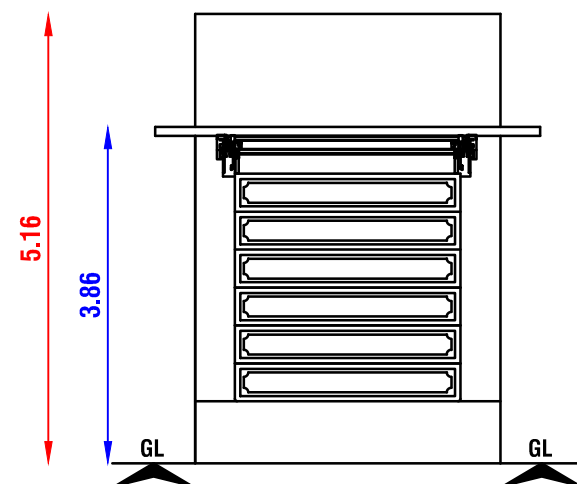
FRONT ELEVATION
