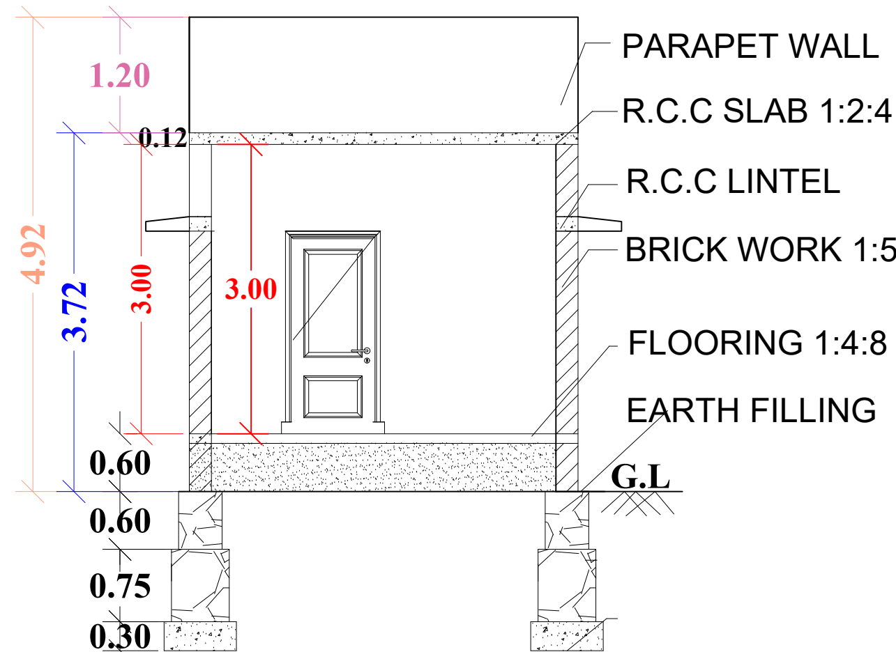
"SECTION "AB"
