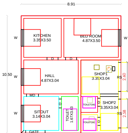
PROPOSED G.F. PLAN
