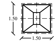
PLAN OF FOOTING
