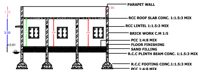
SECTION AB
