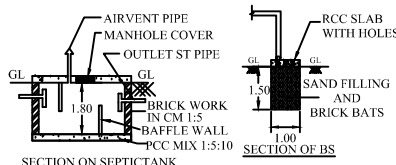
SECTION ON SEPTICTANK
